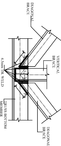
TYPICAL WELDING DETAIL OF BOTTOM MEMBER CONNECTION WITH BRACINGS
