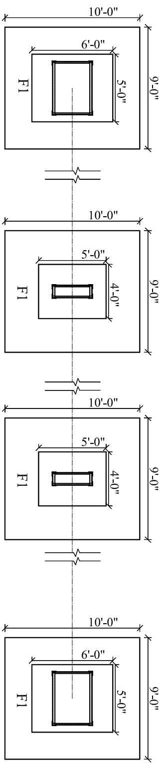
FOUNDATION PLAN
