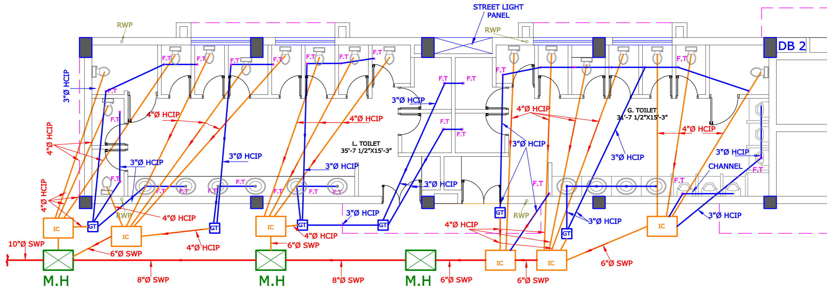
TOILET BLOCK SEWER PLAN
