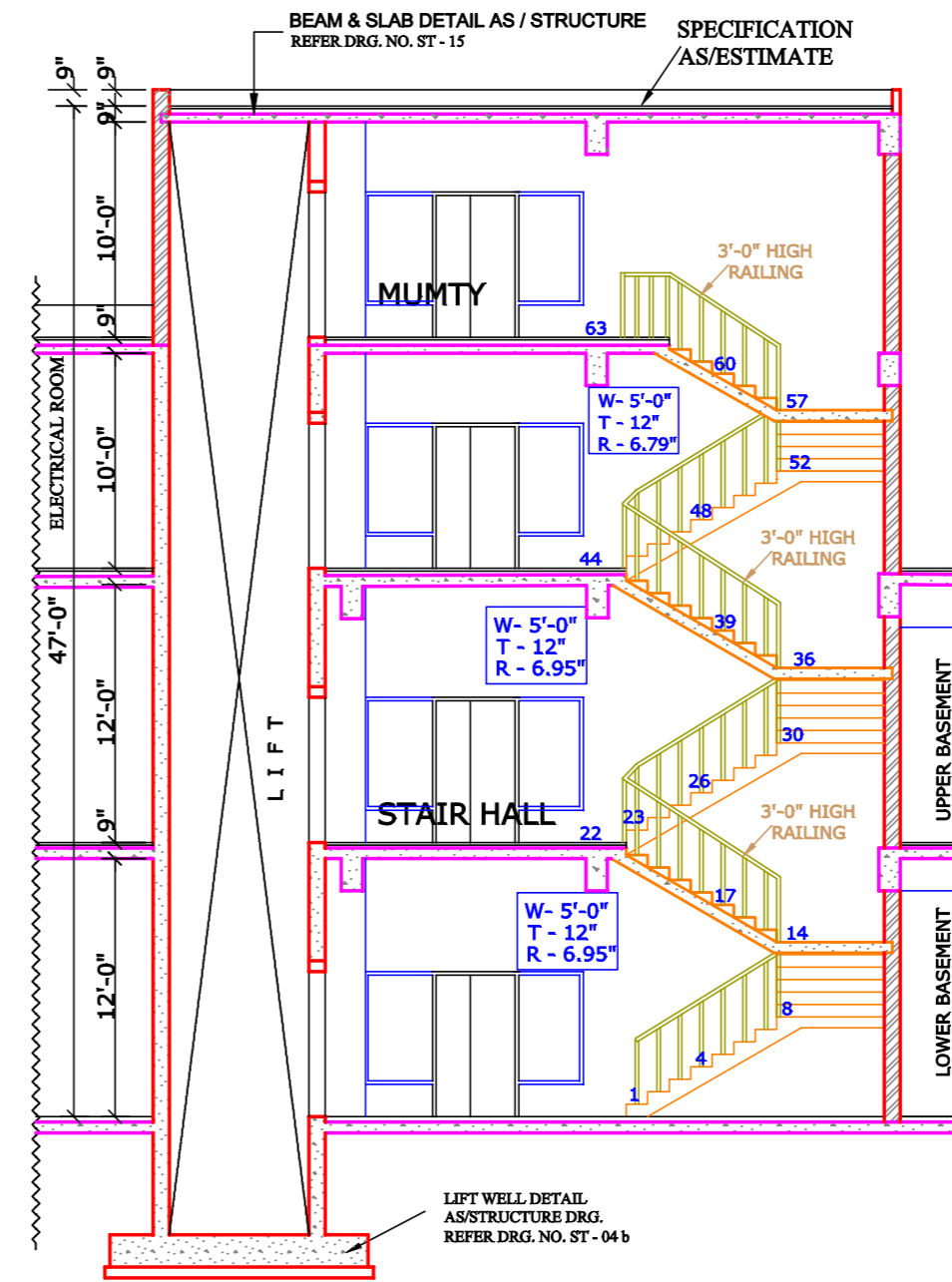
SECTION AT G-G
