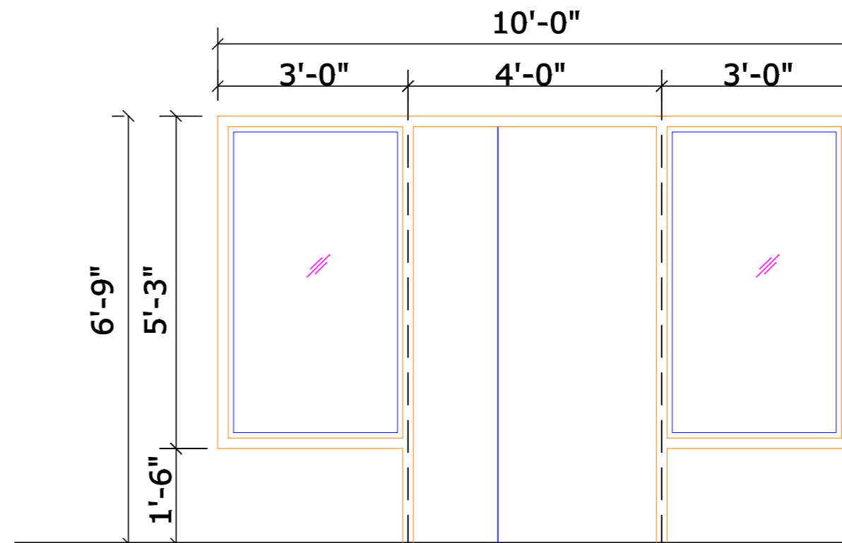
D = 4'-0" X 6'-9" W2 = 3'-0" X 5'-3" STAIR HALL
