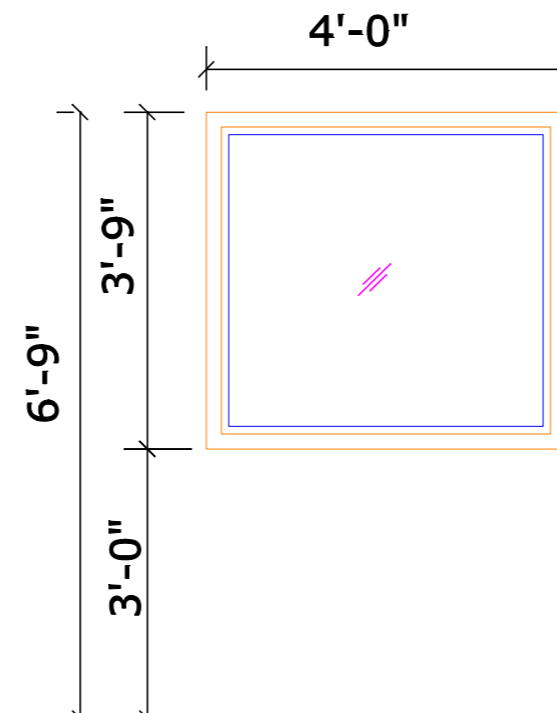
W1 = 4'-0" X 3'-9"
