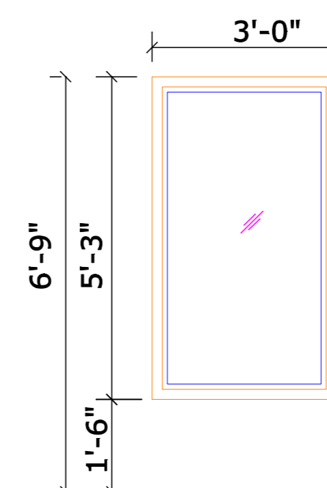
W2 = 3'-0" X 5'-3"
