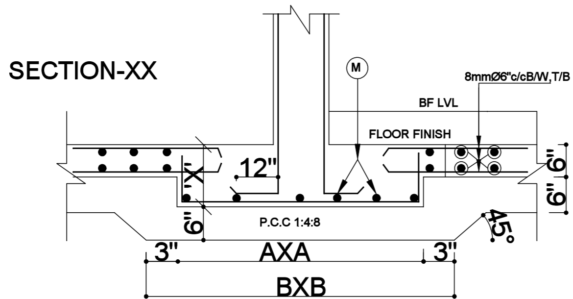
TYPICAL SECTION OF COLUMN FIG-1
