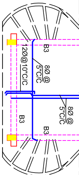
GROUND & FIRST FLOOR SLAB PLAN
