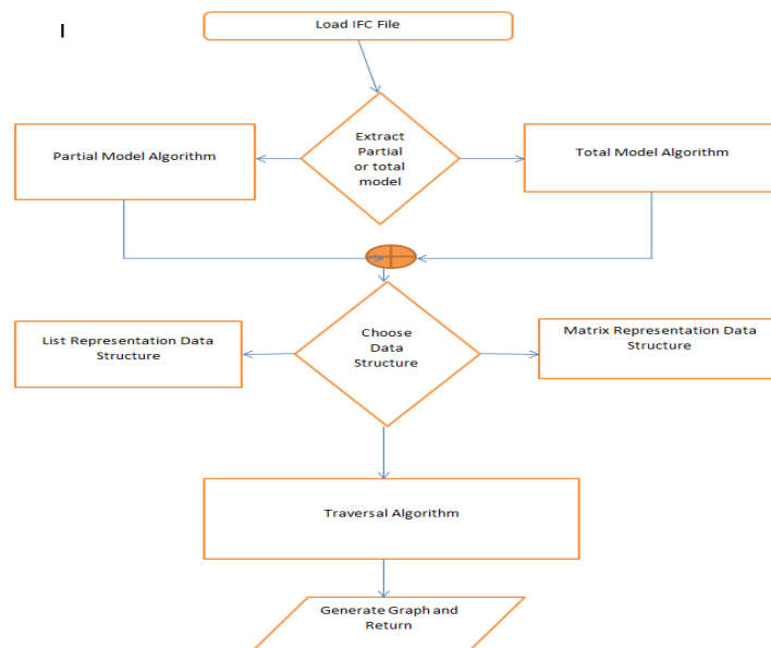
Fig. 2 Flowchart for selecting traversal algorithm
