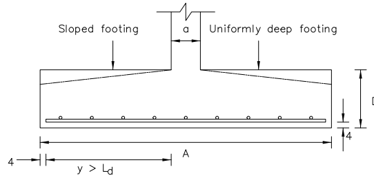
(a) Section of uniformaly and sloped footing
