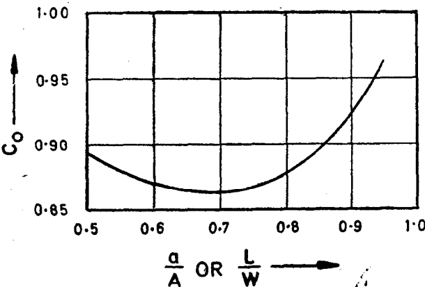
FIG. 1 COEFFICIENT ' C_o ' IN THE ORIFICE FORMULA
