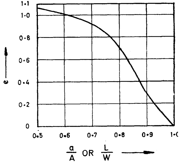
FIG. 2 COEFFICIENT 'e' IN THE ORIFICE FORMULA
