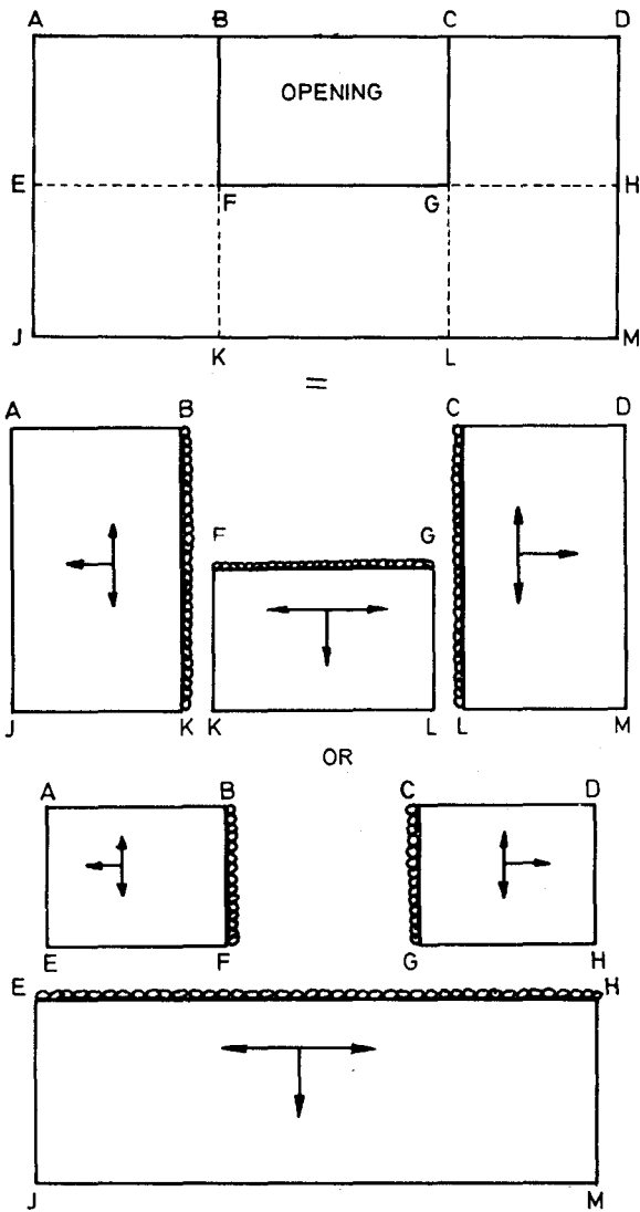
FIG. E-31 DESIGN OF PANEL HAVING A LARGE OPENING
