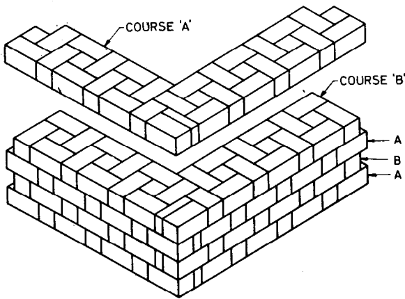
FIG. 3 DOUBLE FLEMISH BOND
