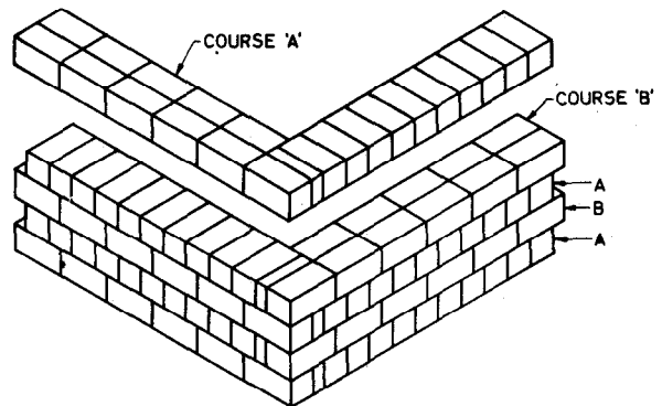
FIG. 2 ENGLISH BOND
