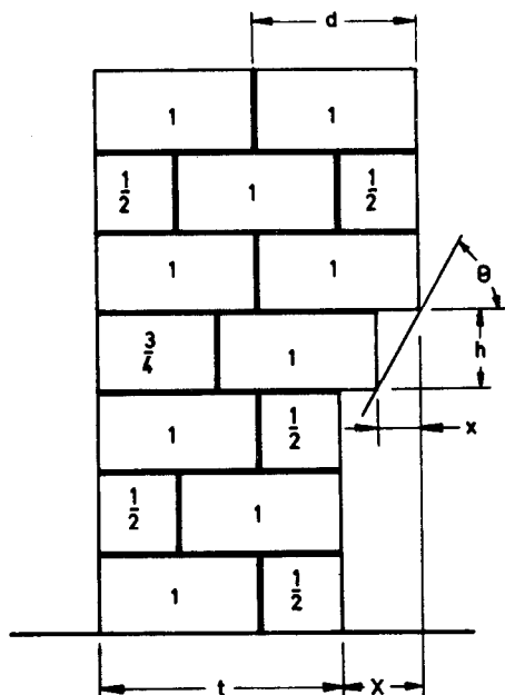
FIG. E-32 LIMITATION OF A CORBEL IN MASONRY
