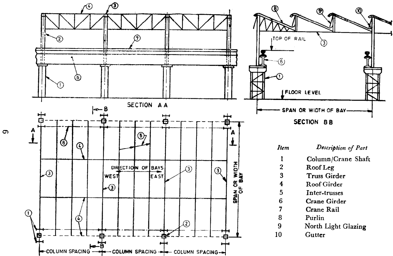
FIG. 2 TYPICAL FACTORY BUILDING — DIRECTION OF BAY, EAST-WEST
