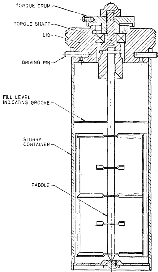
FIG. 1 TYPICAL ATMOSPHERIC PRESSURE CONSISTOMETER
