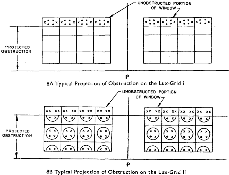
FIG. 8 TYPICAL PROJECTION OF OBSTRUCTION ON THE LUX-GRIDS I & II
