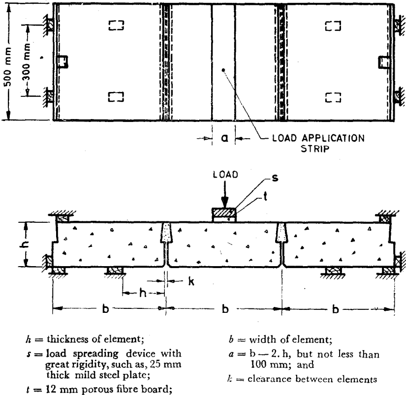
FIG. 1 LOADING ARRANGEMENT FOR JOINTED ELEMENTS OF CELLULAR CONCRETE
