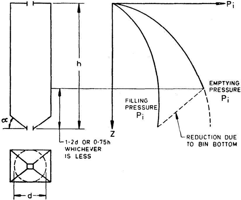
FIG. 3 PRESSURE VARIATION ALONG BIN DEPTH
