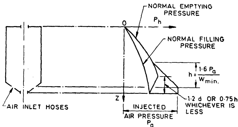
FIG. 4 PRESSURE SCHEME DURING PNEUMATIC EMPTYING
