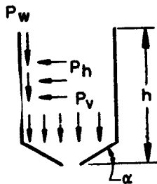
FIG. 2 BIN LOADS
