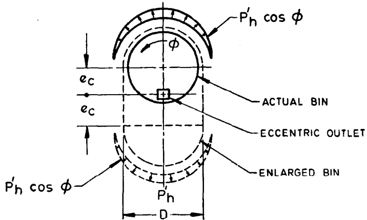
5B CIRCULAR BIN
