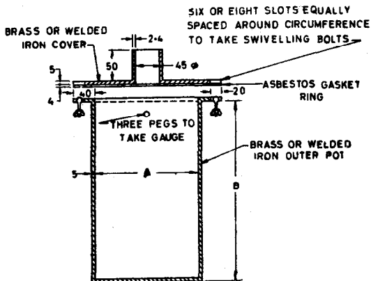
A — From 125 mm to 225 mm \phi as appropriate B — From 200 mm to 375 mm \phi as appropriate All dimensions in millimetres.
