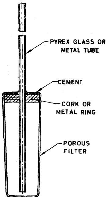
FIG. 1 ASSEMBLY OF FILTER FOR THE DETERMINATION OF THE BITUMINOUS STABILIZER CONTENT OF STABILIZED SOILS
