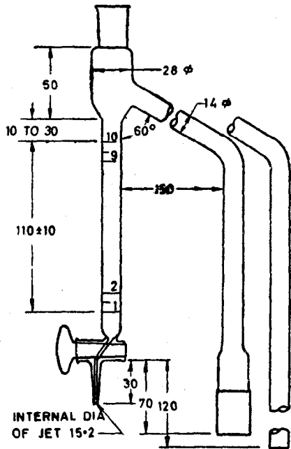
FIG. 7 10 ml RECEIVER SHOWING ALTERNATIVE CONNECTIONS TO DISTILLATION VESSEL
