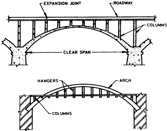
FIG. 3 CLASSIFICATION OF CONCRETE ARCHES BASED ON CONSTRUCTION — TYPICAL OPEN SPANDEL ARCH
