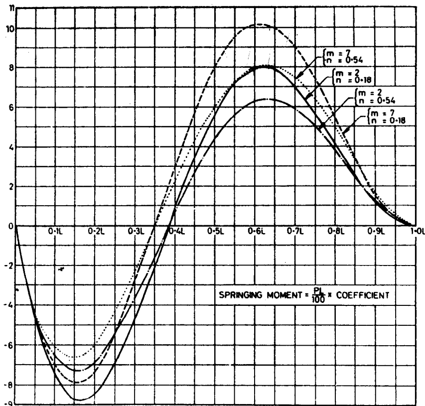
FIG. 10 INFLUENCE LINES FOR MOMENT AT SPRINGING
