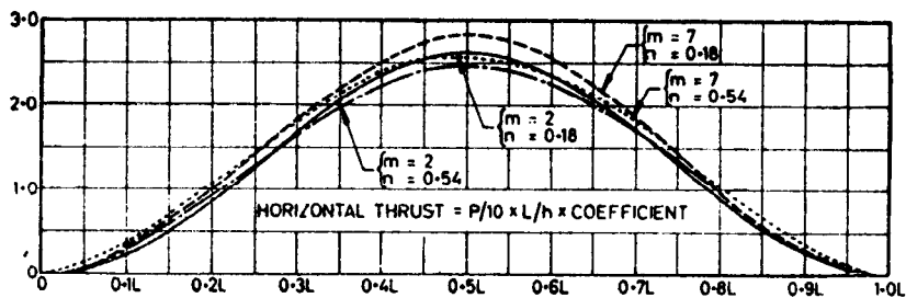
FIG. 11 INFLUENCE LINES FOR HORIZONTAL THRUST AT CROWN
