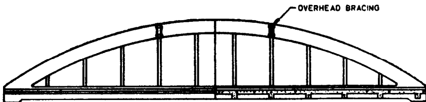
FIG. 4 CLASSIFICATION OF CONCRETE ARCHES BASED ON CONSTRUCTION -- TYPICAL TIED ARCH OR BOW-STRINGS GIRDER
