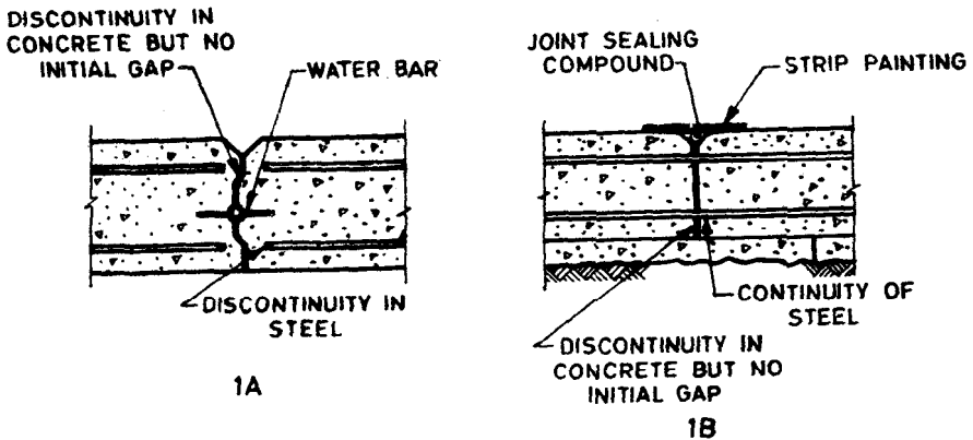
FIG. 1 TYPICAL CONTRACTION JOINTS
