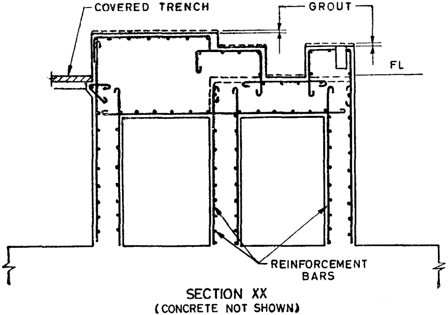
FIG. 2 TYPICAL FOUNDATION FOR PRIMARY AIR FAN
