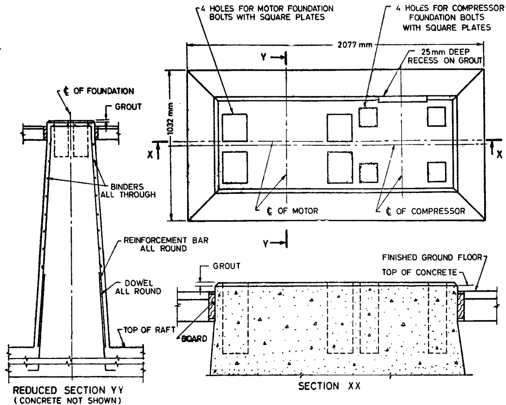
FIG. 3 TYPICAL FOUNDATION FOR INSTRUMENT AIR COMPRESSOR
