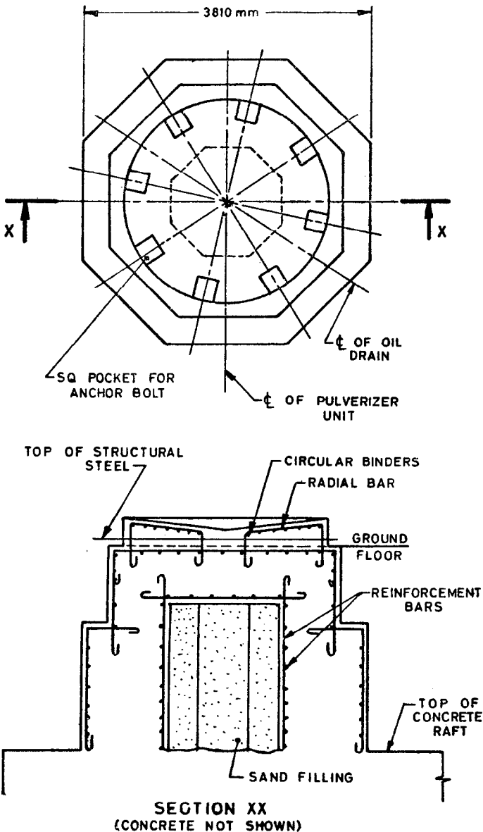
FIG. 1 TYPICAL FOUNDATION FOR CRUSHING MILL (PULVERIZER UNIT)
