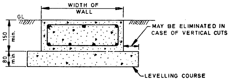
3B BEAM IN NON-EXPANSIVE SOILS
