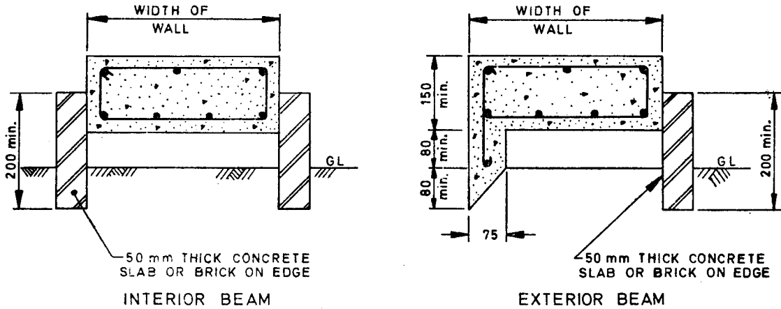
3A BEAMS IN EXPANSIVE SOILS
