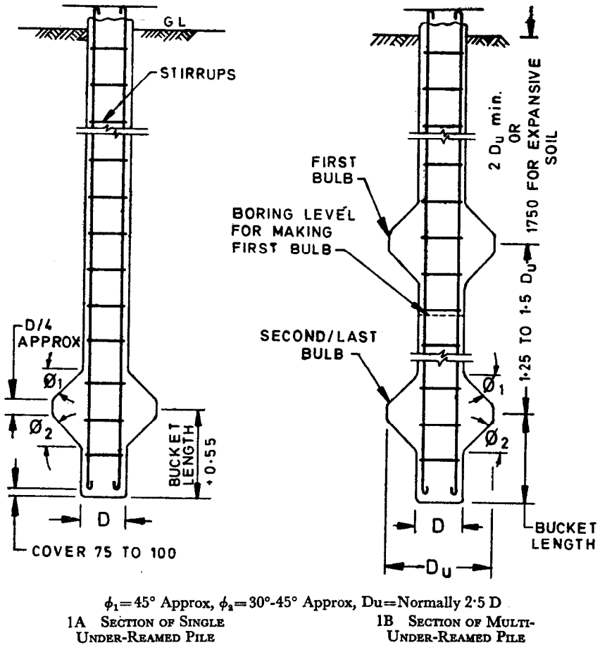
FIG. 1 TYPICAL DETAILS OF BORED CAST in situ UNDER-REAMED PILE FOUNDATIONS
