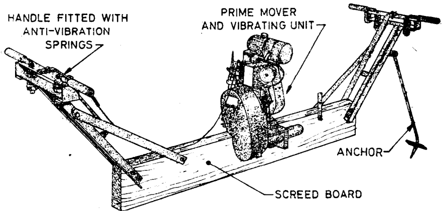
FIG. 1 TYPICAL SKETCH OF SCREED BOARD CONCRETE VIBRATOR
