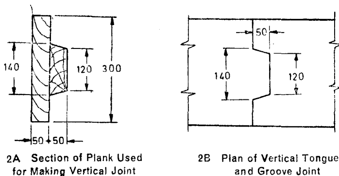
FIG. 2 TYPICAL DETAILS OF CONSTRUCTION JOINT IN In Situ SOIL-CEMENT WALLS OF 300 mm THICKNESS
