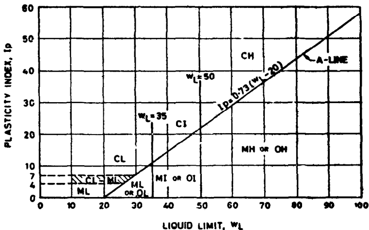
FIG. 1 PLASTICITY CHART
