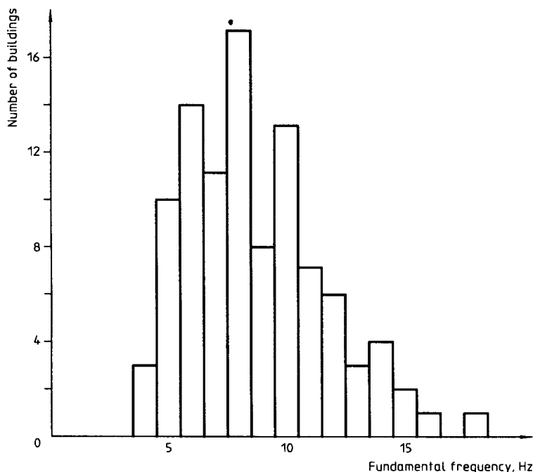
Figure D.3 — Frequencies measured in 96 low-rise buildings
