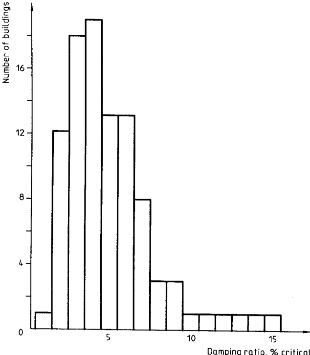
Figure D.4 — Damping ratios measured in 96 low-rise buildings
