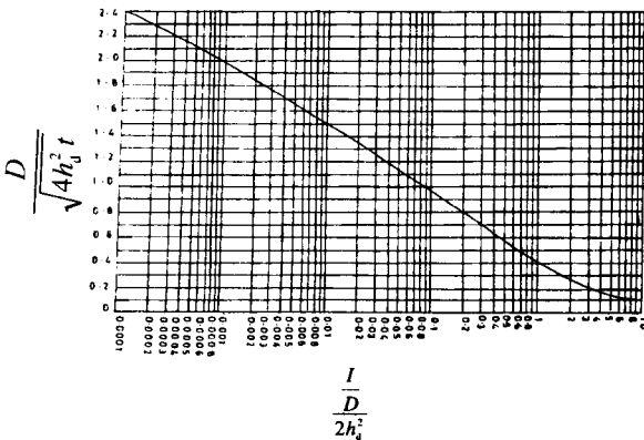
FIG. 2 PLOT OF \frac{I}{\frac{D}{2h_d^2}} VS \frac{D}{\sqrt{4h_d^2 t}}
