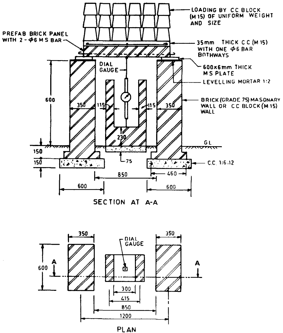
All dimensions in millimetres. FIG. 3 A TYPICAL LOAD TEST SETUP
