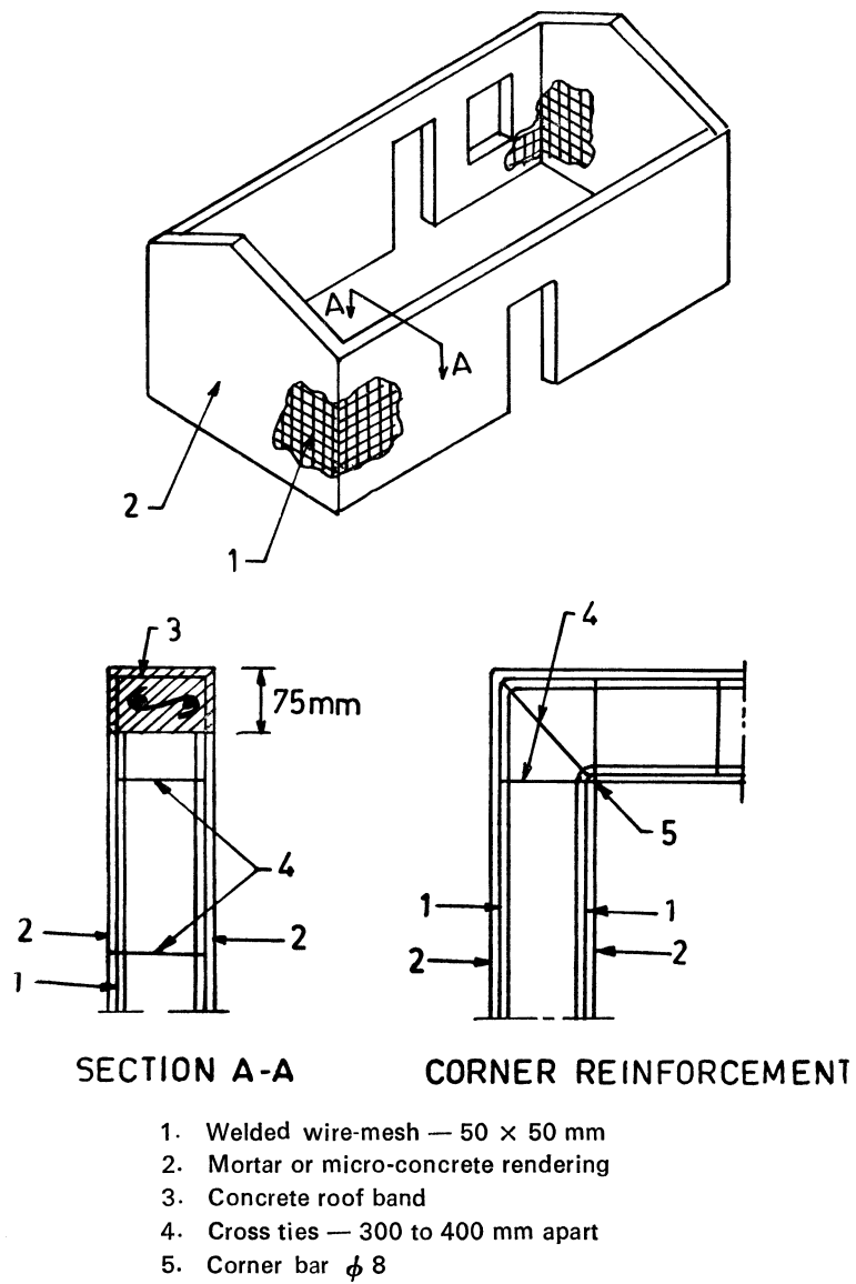
FIG. 9 STRENGTHENING WITH WIRE-MESH AND MORTAR
