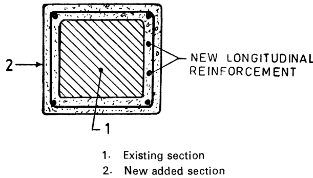
FIG. 15 CASING A CONCRETE COLUMN
