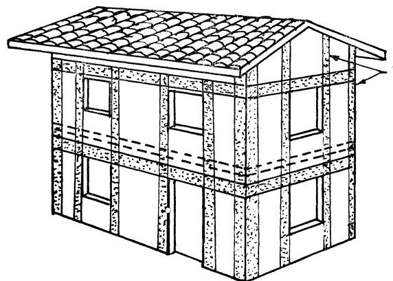
FIG. 11 STRENGTHENING OF WALLS BY PRESTRESSING
