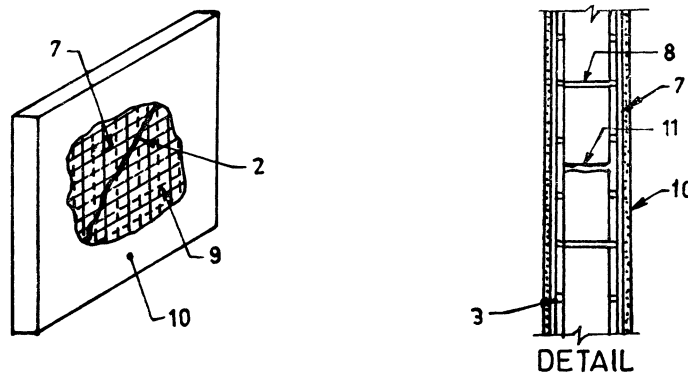
1C Cement mortar and wire mesh in cracks
