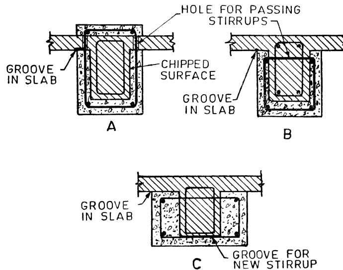
FIG. 16 INCREASING THE SECTION AND REINFORCEMENT OF EXISTING BEAMS
