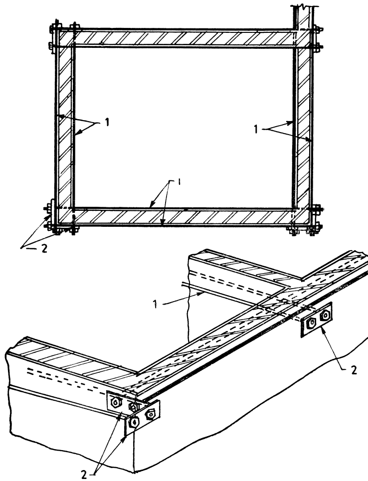
FIG. 11 STRENGTHENING OF WALLS BY PRESTRESSING
