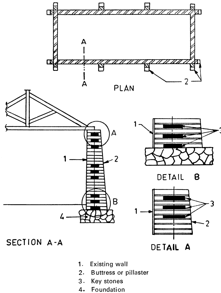
FIG. 14 STRENGTHENING OF LONG WALLS BY BUTTRESSES
