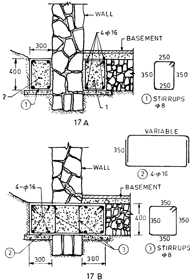
FIG. 17 STRENGTHENING EXISTING FOUNDATION (R. C. STRIP ON BOTH SIDES)
