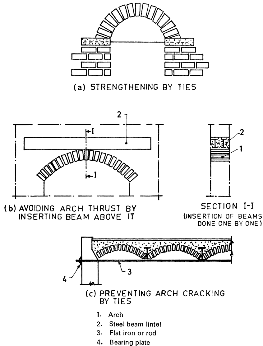
FIG. 13 STRENGTHENING AN ARCHED OPENING IN MASONRY WALL
