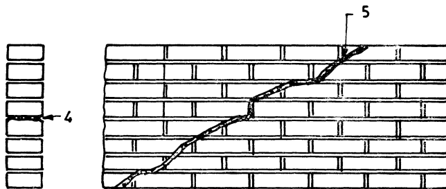
1A Grout or epoxy injection in cracks
