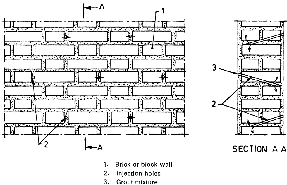
FIG. 8 GROUT OR EPOXY INJECTION IN EXISTING WEAK WALLS
