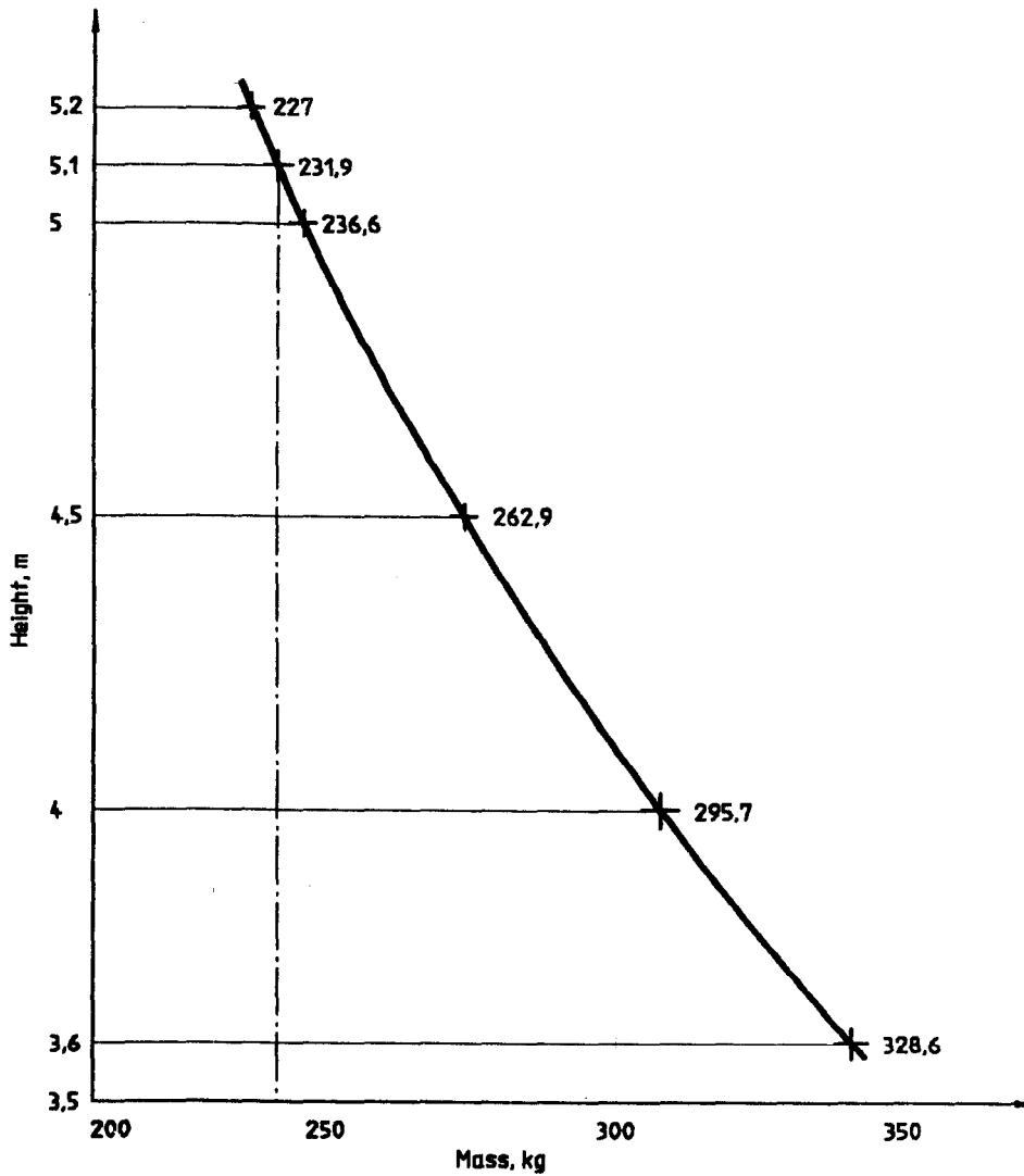
Figure 3 — Height and mass for drop test object with capability of developing energy of 11 600 J
