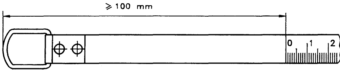
FIG. 2 MEASURE WITH ZERO AWAY FROM RING
