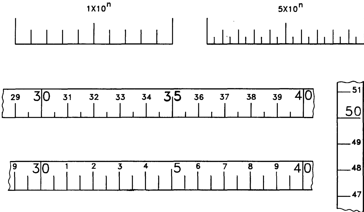
FIG. 3 GRADUATION LINES AND NUMBERING
