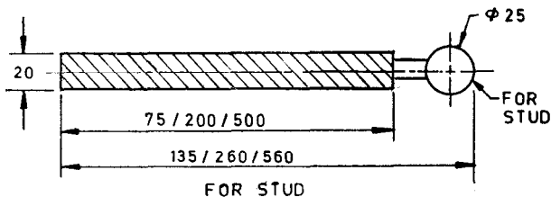
2A PERMANENT REFERENCE STUD/ HOOK ANCHOR
