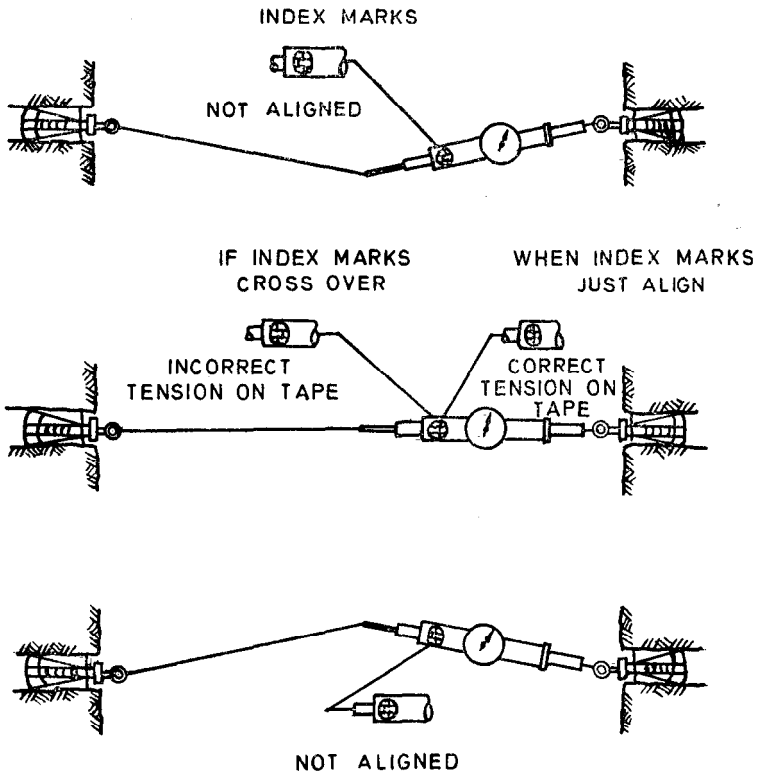
FIG. 4 ALIGNMENT PATTERN OF TAPE EXTENSOMETER
