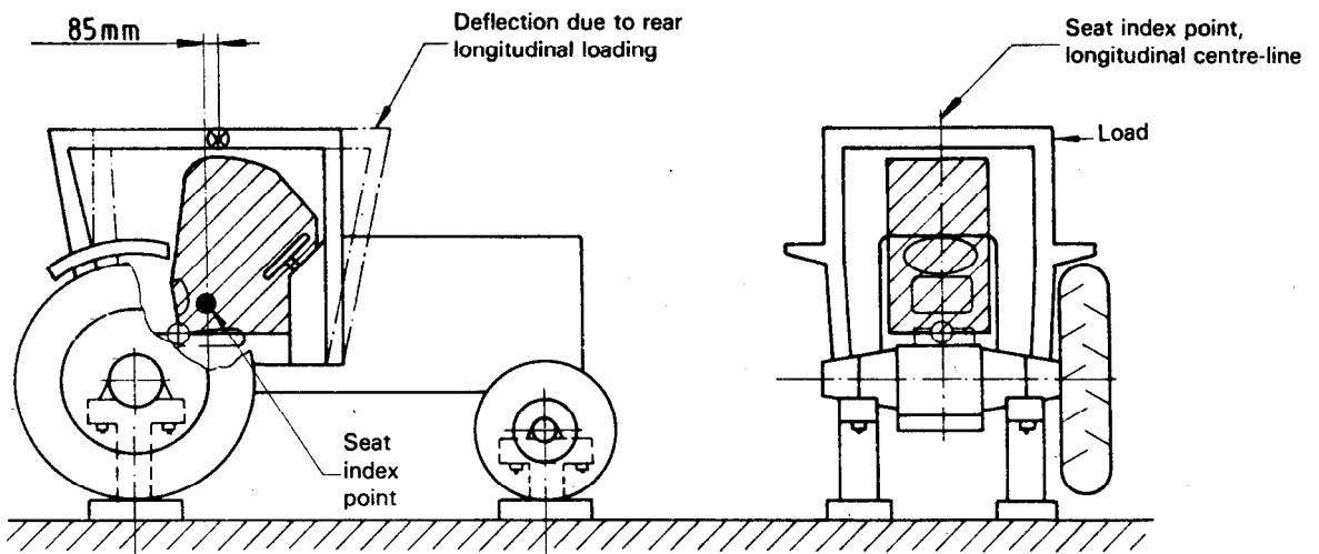
Figure 3 – Side load application
