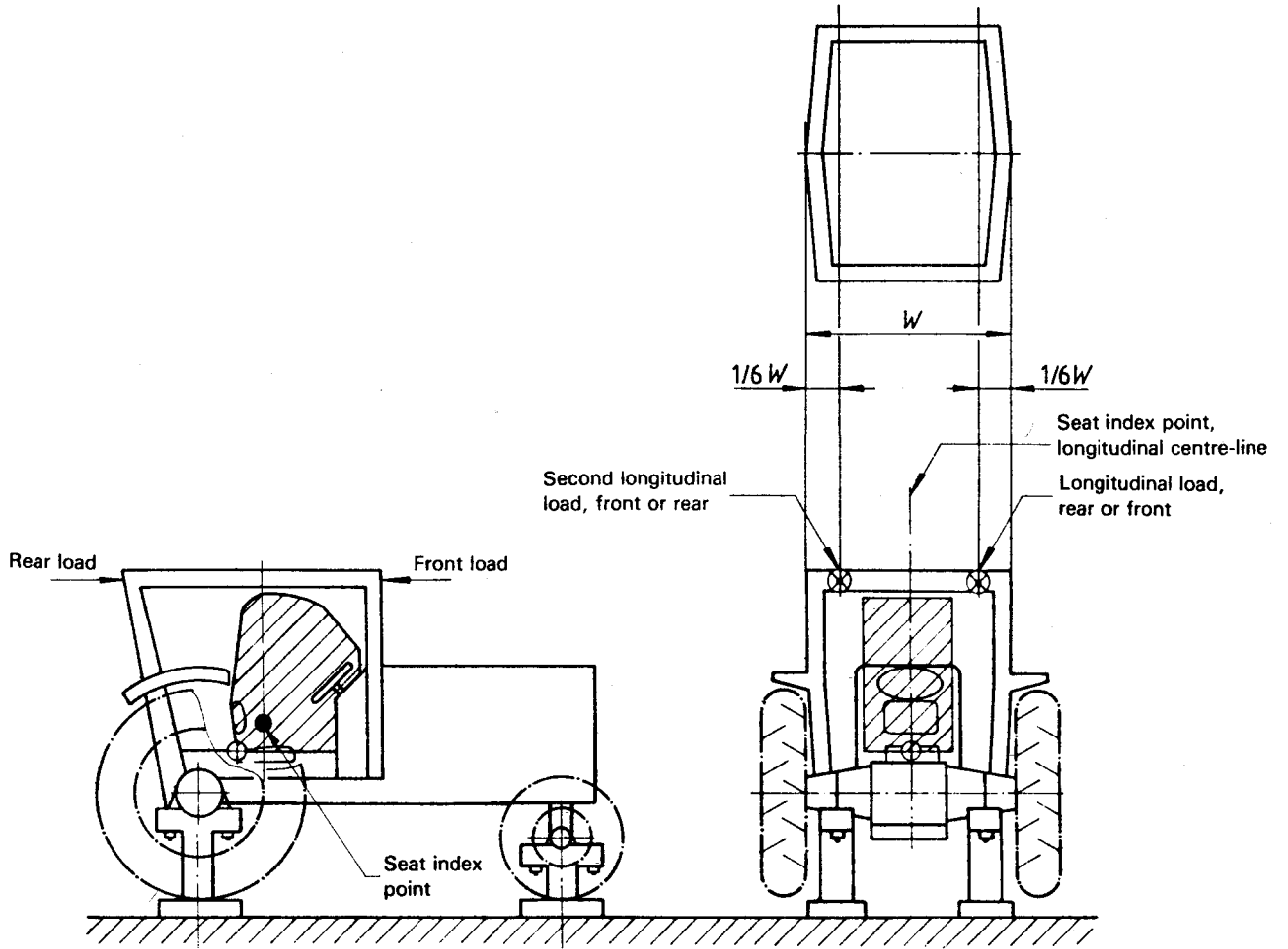
Figure 2 – Front and rear load application
