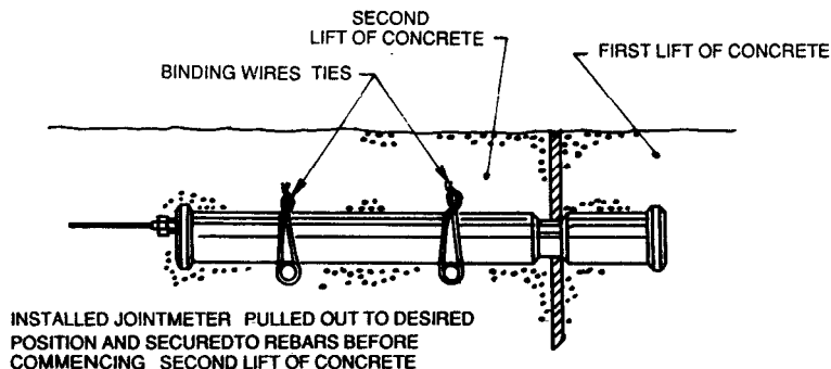
FIG. 1 JOINTMETER INSTALLATION
